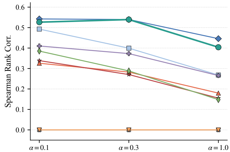
(c) Spearman Rank Correlation \uparrow
