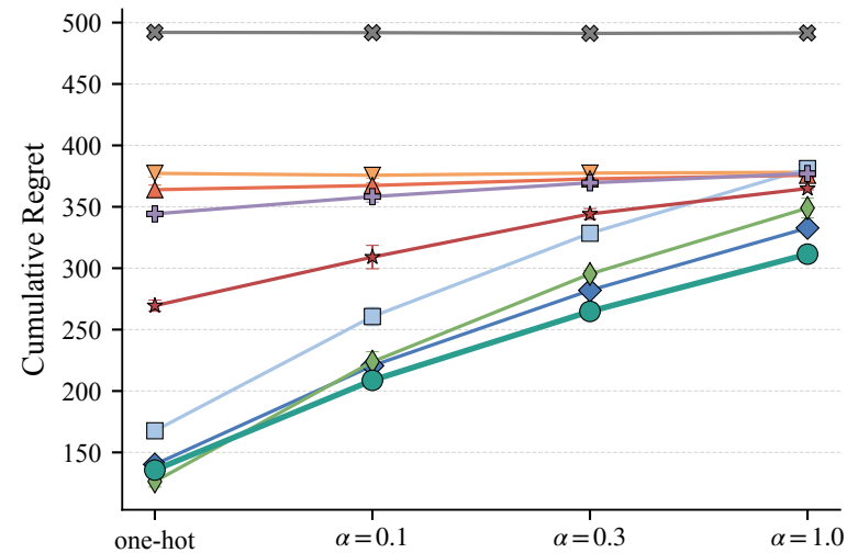
(a) Cumulative Regret \downarrow
