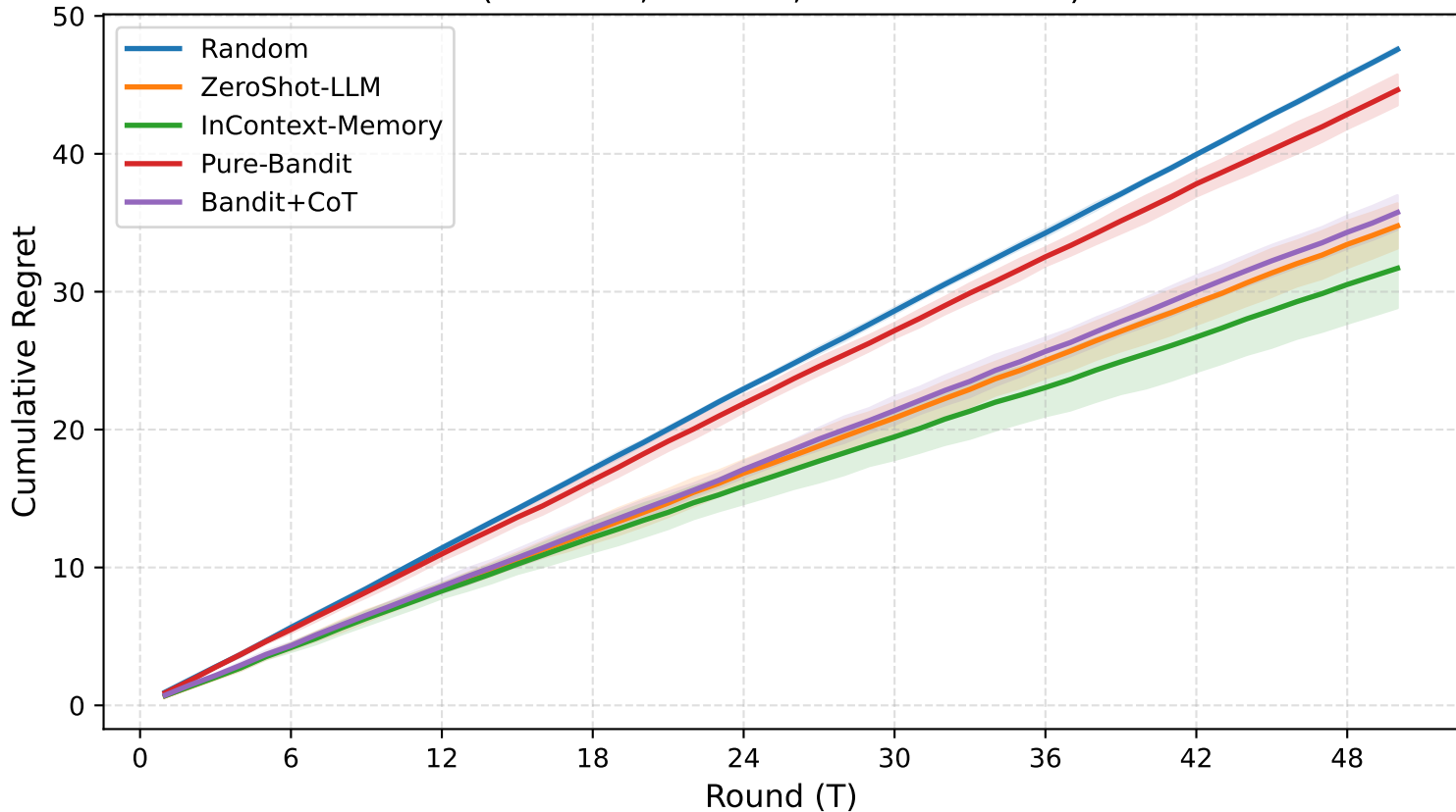
Cumulative Regret over Time (20 users, 5 seeds, 95% CI shaded)
