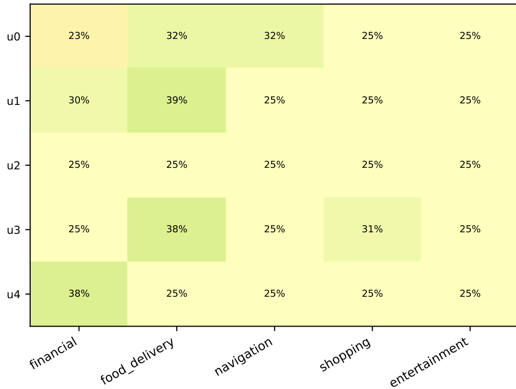
Pure-Bandit
