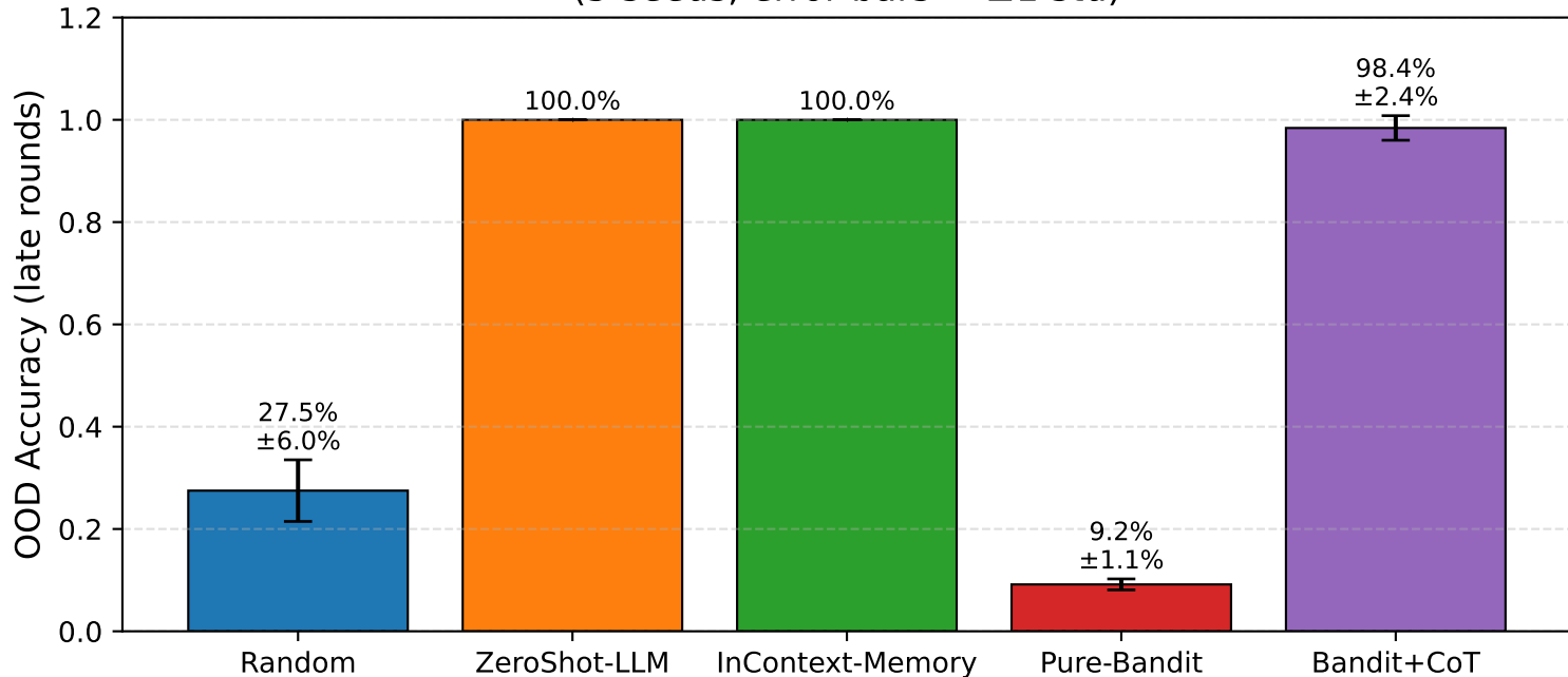
OOD Robustness — Late Rounds (after round 60\% \times T ) (5 seeds, error bars = \pm 1 std)
