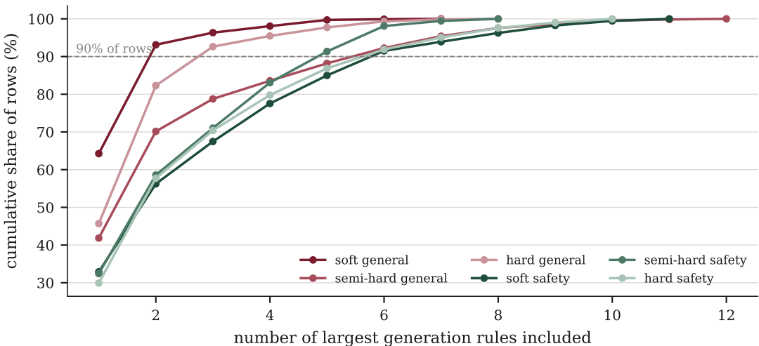
Concentration of the synthetic corpus in a handful of rules
