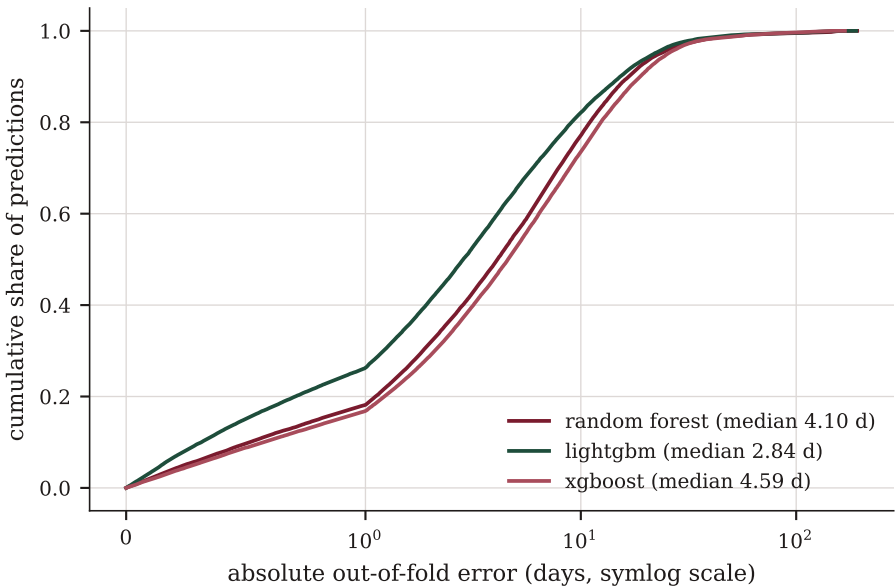
Out-of-fold error distribution, all 34\,000 rows per model
