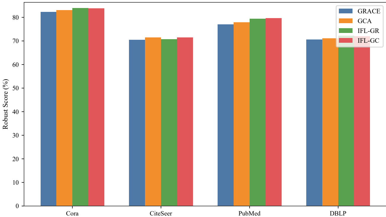
Robust Score
