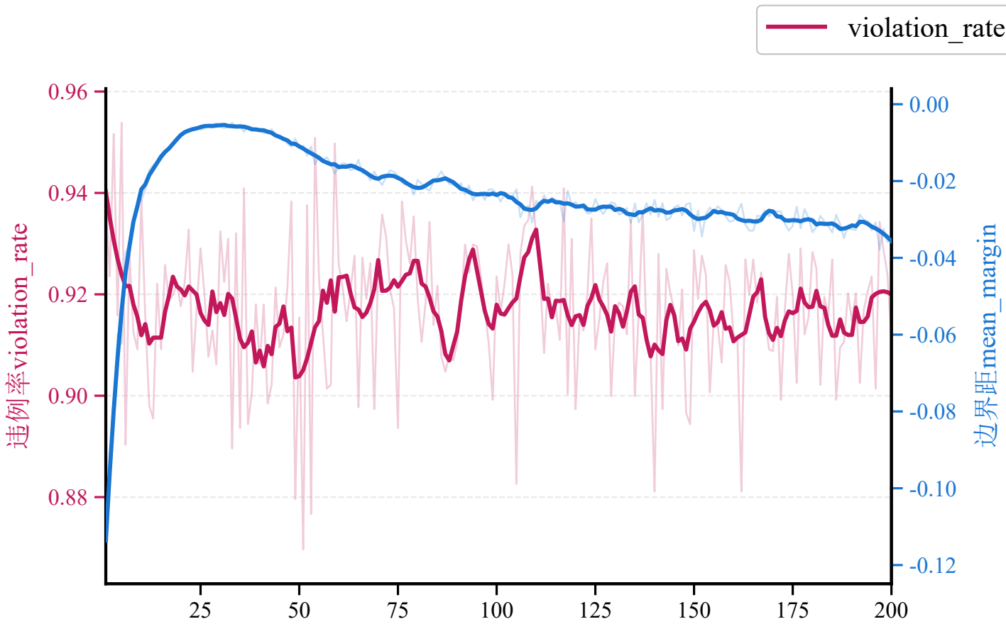
(a) Cora
