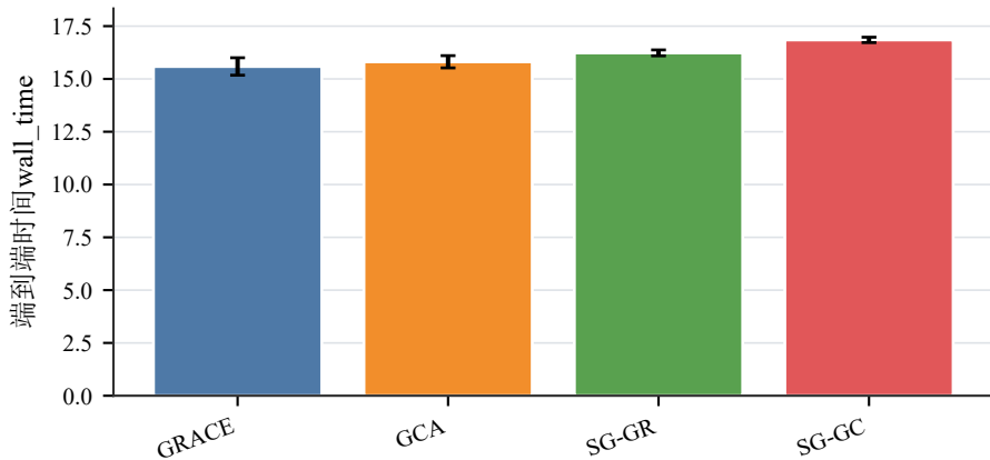
(a) Cora
