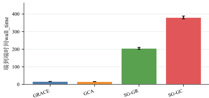
(c) PubMed
