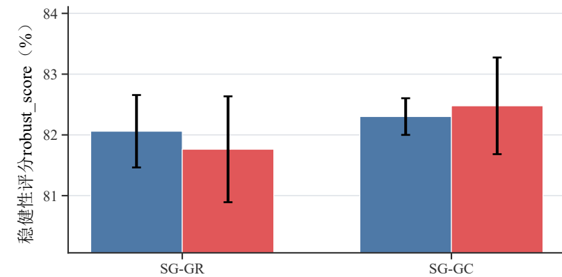
(a) Cora
