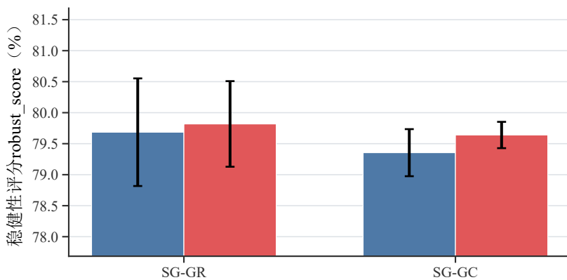
(c) PubMed
