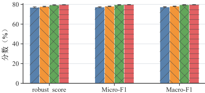
(c) PubMed
