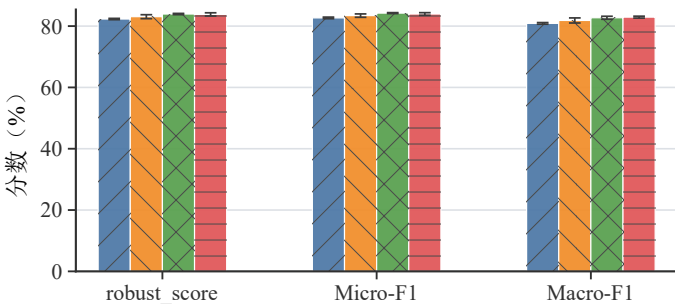
(a) Cora
