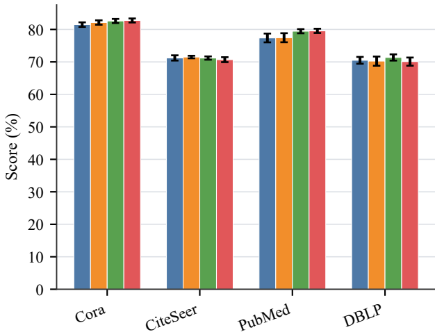
robust_score
