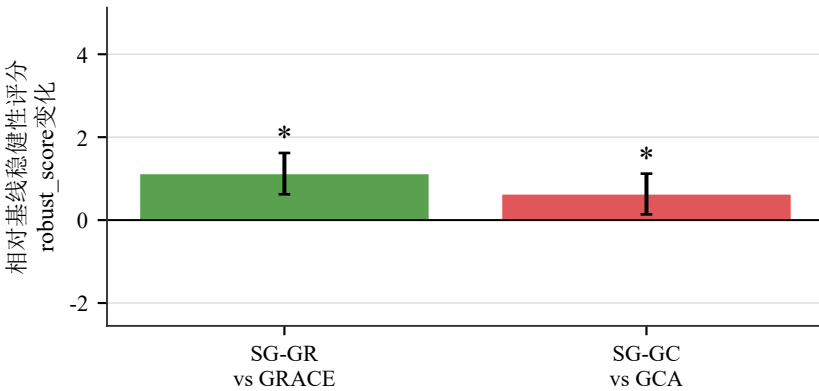
(a) Cora
