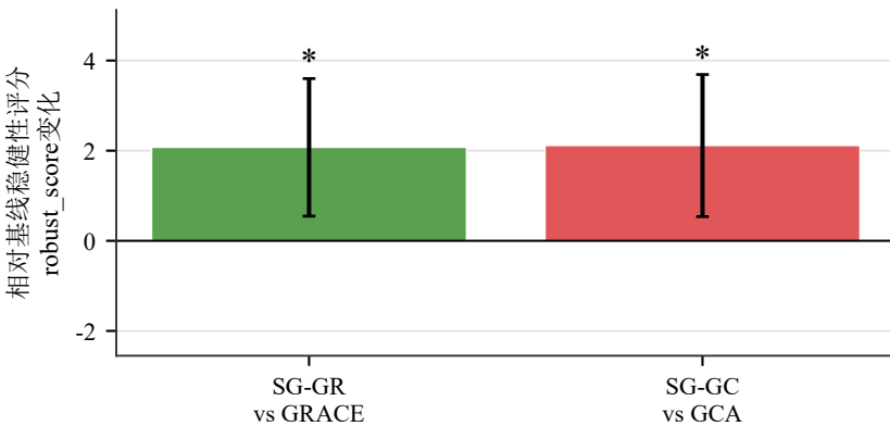
(c) PubMed
