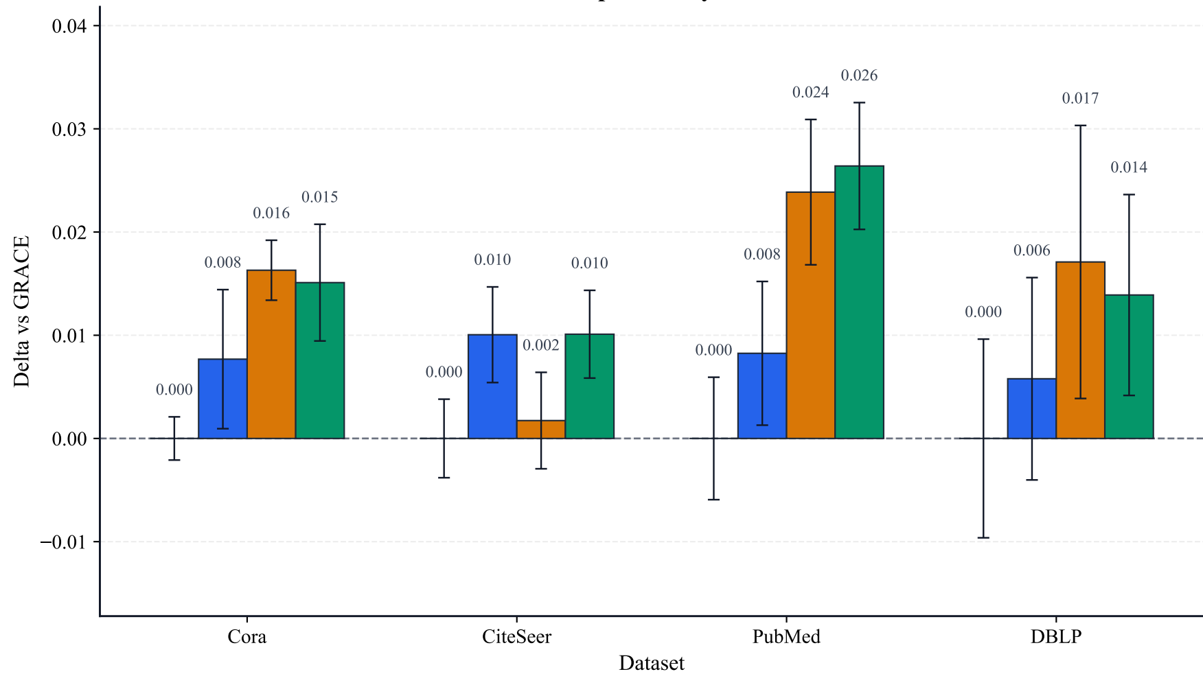
GRACE GCA IFL-GR IFL-GC Performance Comparison by Delta vs GRACE
