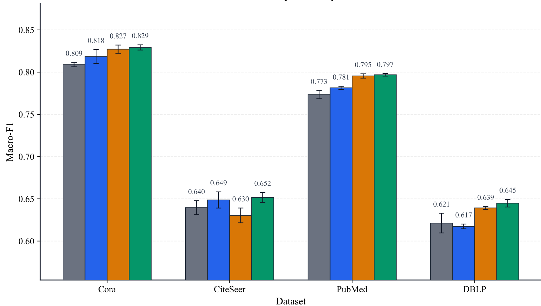
GRACE GCA IFL-GR IFL-GC Performance Comparison by Macro-F1
