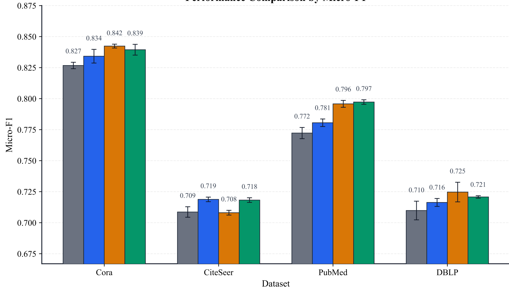
GRACE GCA IFL-GR IFL-GC Performance Comparison by Micro-F1
