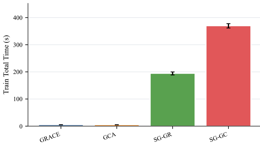
PubMed
