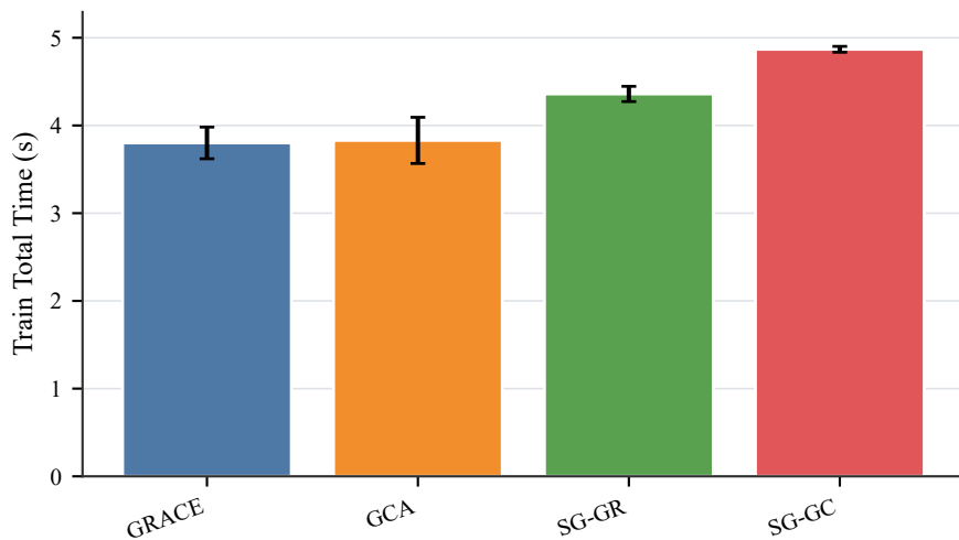
PubMed
