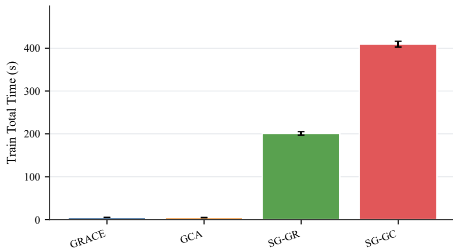
DBLP
