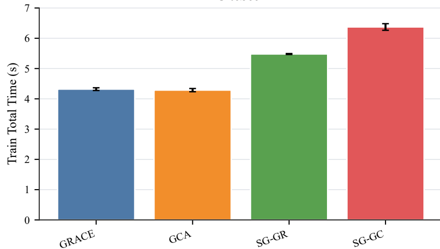
DBLP
