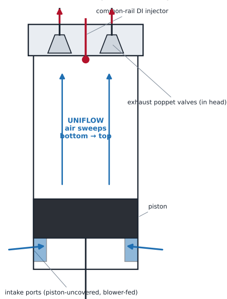
Figure 4: The 2.5L I5 two-stroke uniflow diesel: cylinder cross-section and gas-path.
