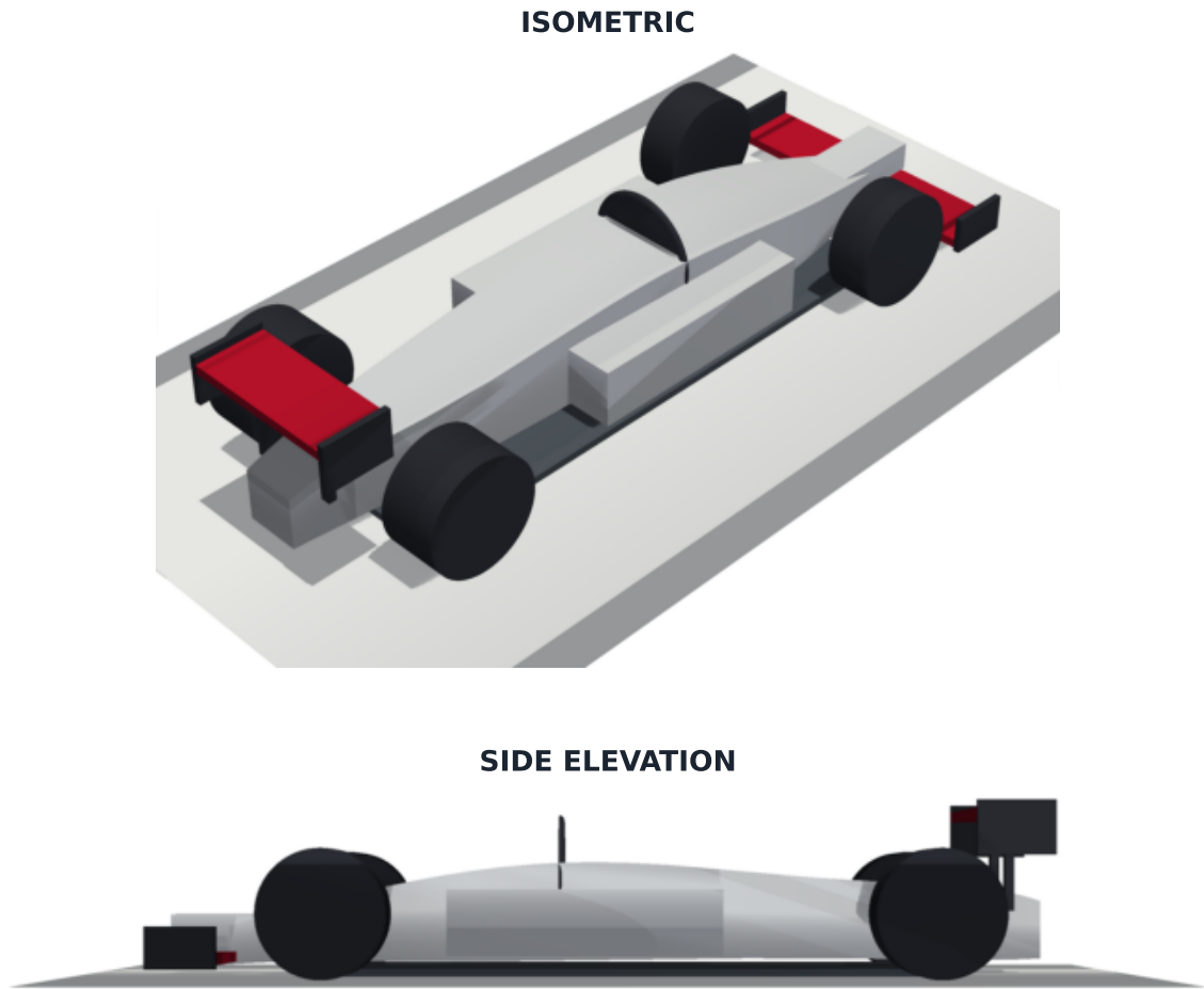
Figure 3: The same parametric solid as a lit 3D render (CadQuery model → STEP; PyVista).
