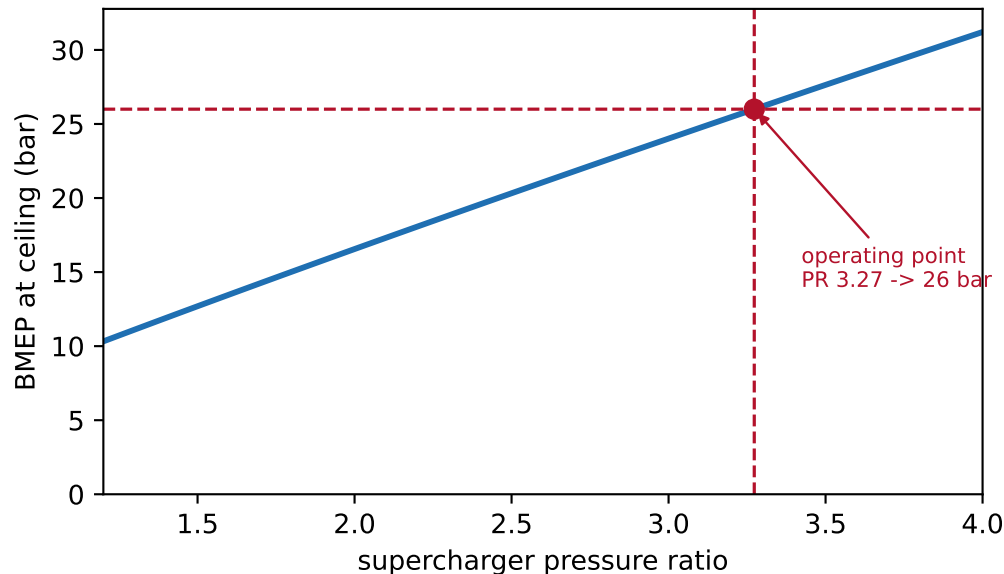
Boost needed for 26 bar BMEP
