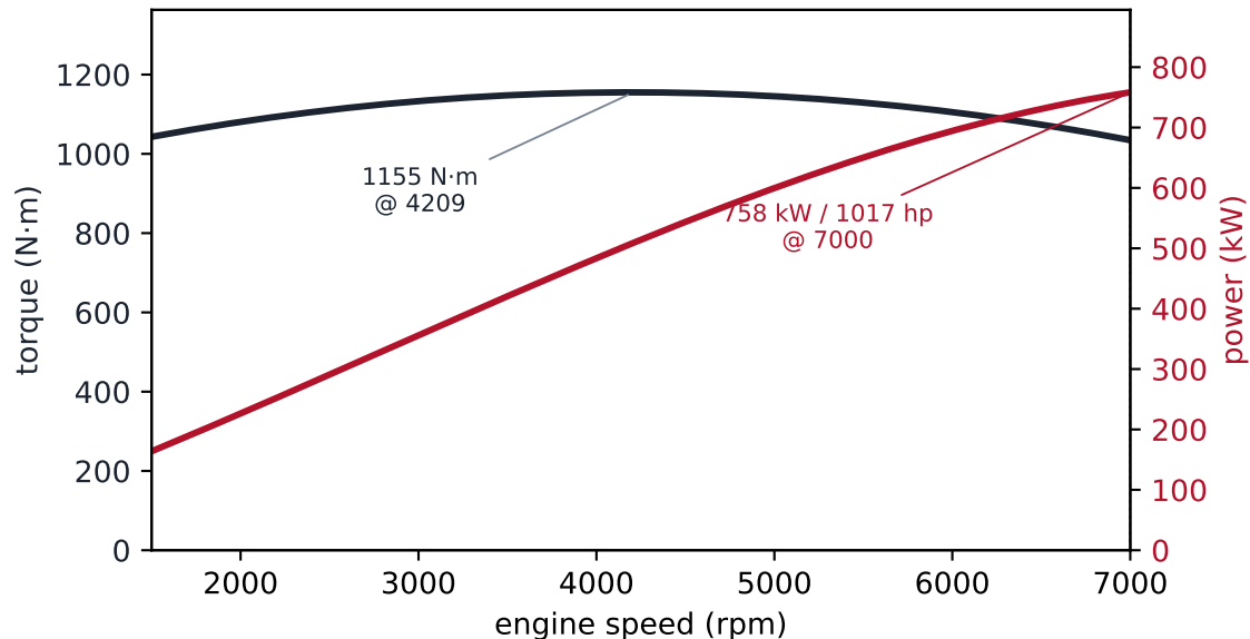
Performance map (screw-blown, flat boost)
