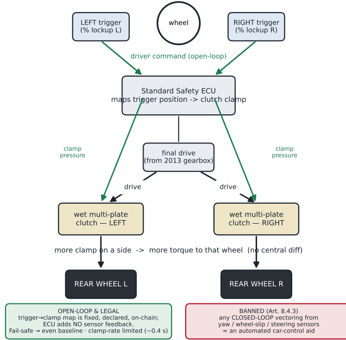
Figure 5: The driver-vectoring twin wet-clutch differential and its open-loop control law.
