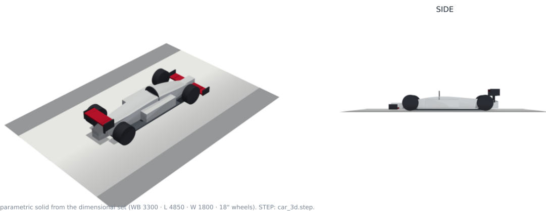
Figure 3: The same parametric solid as a lit 3D render (CadQuery model → STEP; PyVista).
