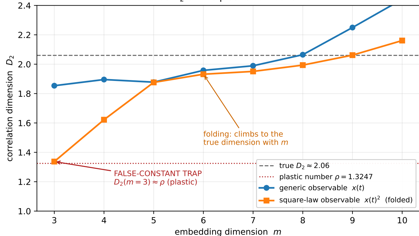
Ptyche: a non-generic (square-law) sensor folds the attractor and lands D_2 on the plastic number at low m
