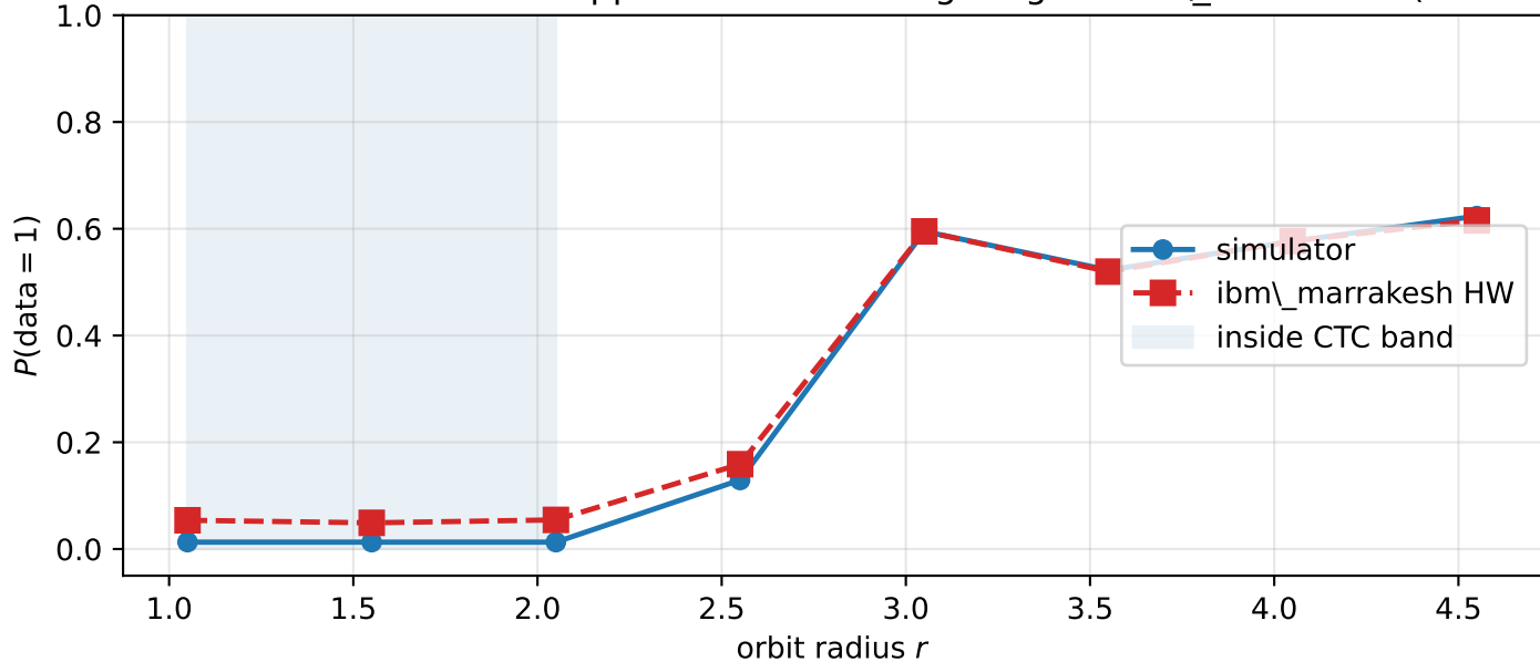
Hardware confirmation: Knopp Drive CTC-band gating on ibm\_marrakesh (batch 6)
