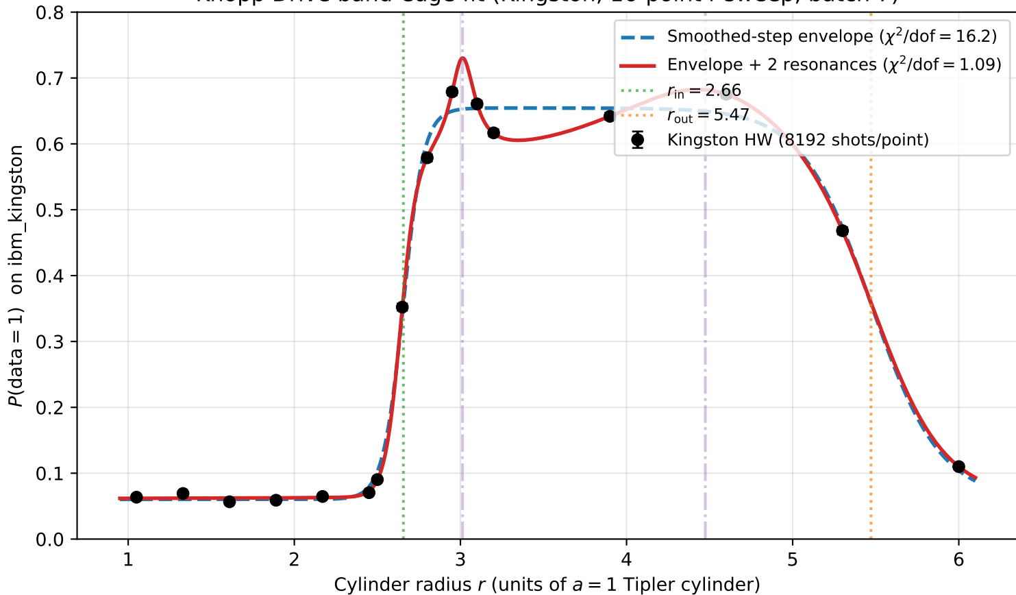
Knopp Drive band-edge fit (Kingston, 16-point r-sweep, batch 7)
