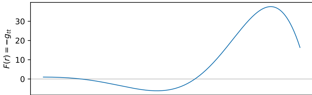
Tipler sinusoid: a = \omega R = 1 , \alpha = \sqrt{3}
