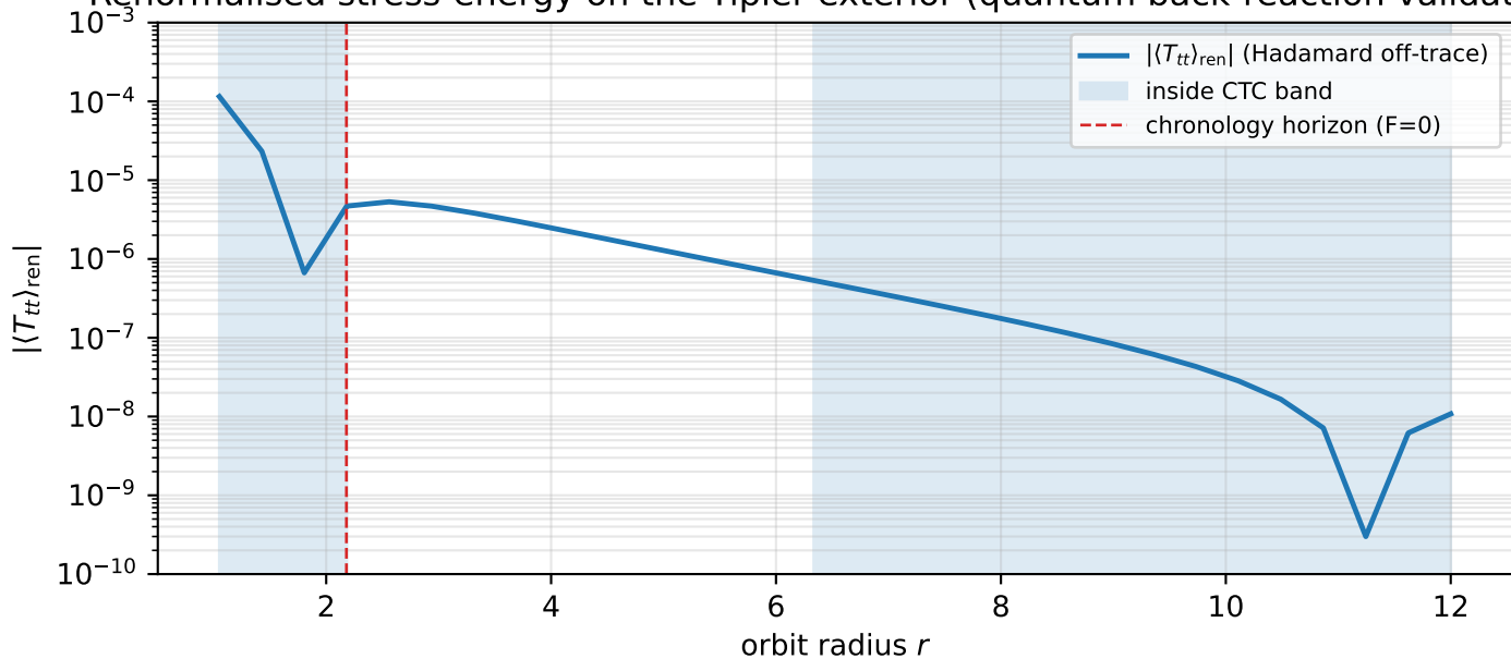
Renormalised stress-energy on the Tipler exterior (quantum back-reaction validation)
