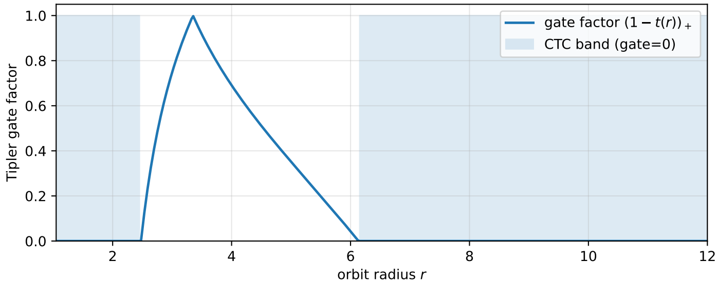
Tipler CTC-band gating: exotic matter is forced to zero inside each band ( \omega = 1, R = 1 )
