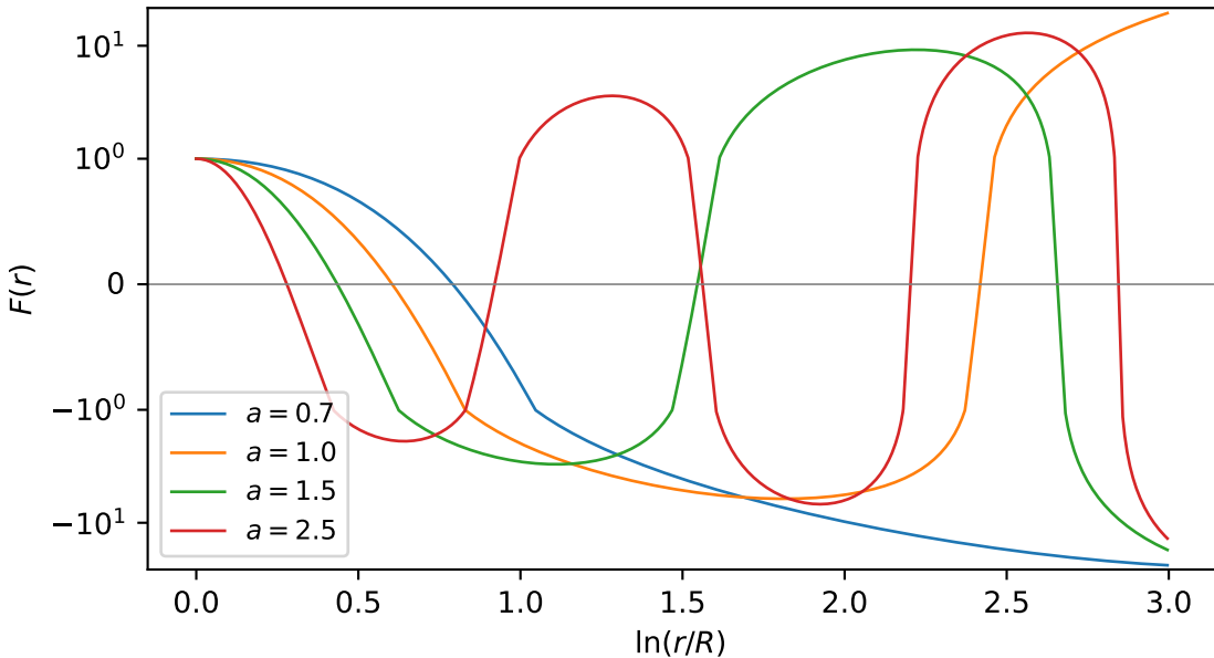
Regime-dispatching robust solver: machine precision at any a
