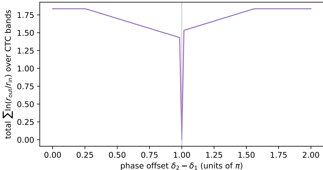
Off-set Tipler sinusoid: CTC log-measure vs phase offset
