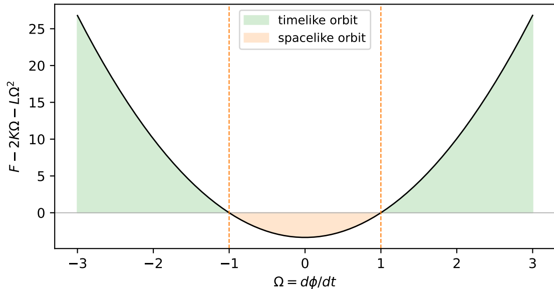
Timelike-orbit sector at r = 3.352 (CTC band 1, a = 1 )
