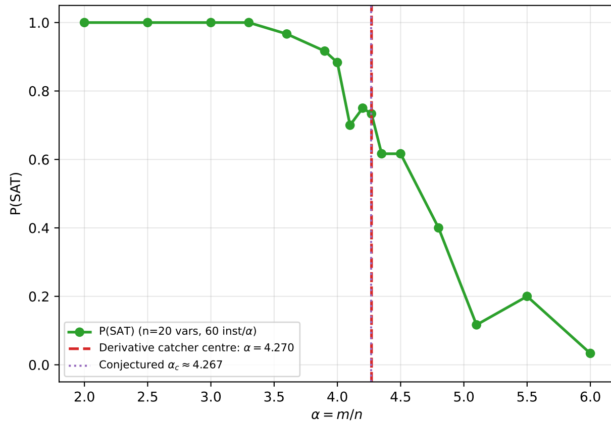
B: 3-SAT phase transition — catcher recovers \alpha_c
