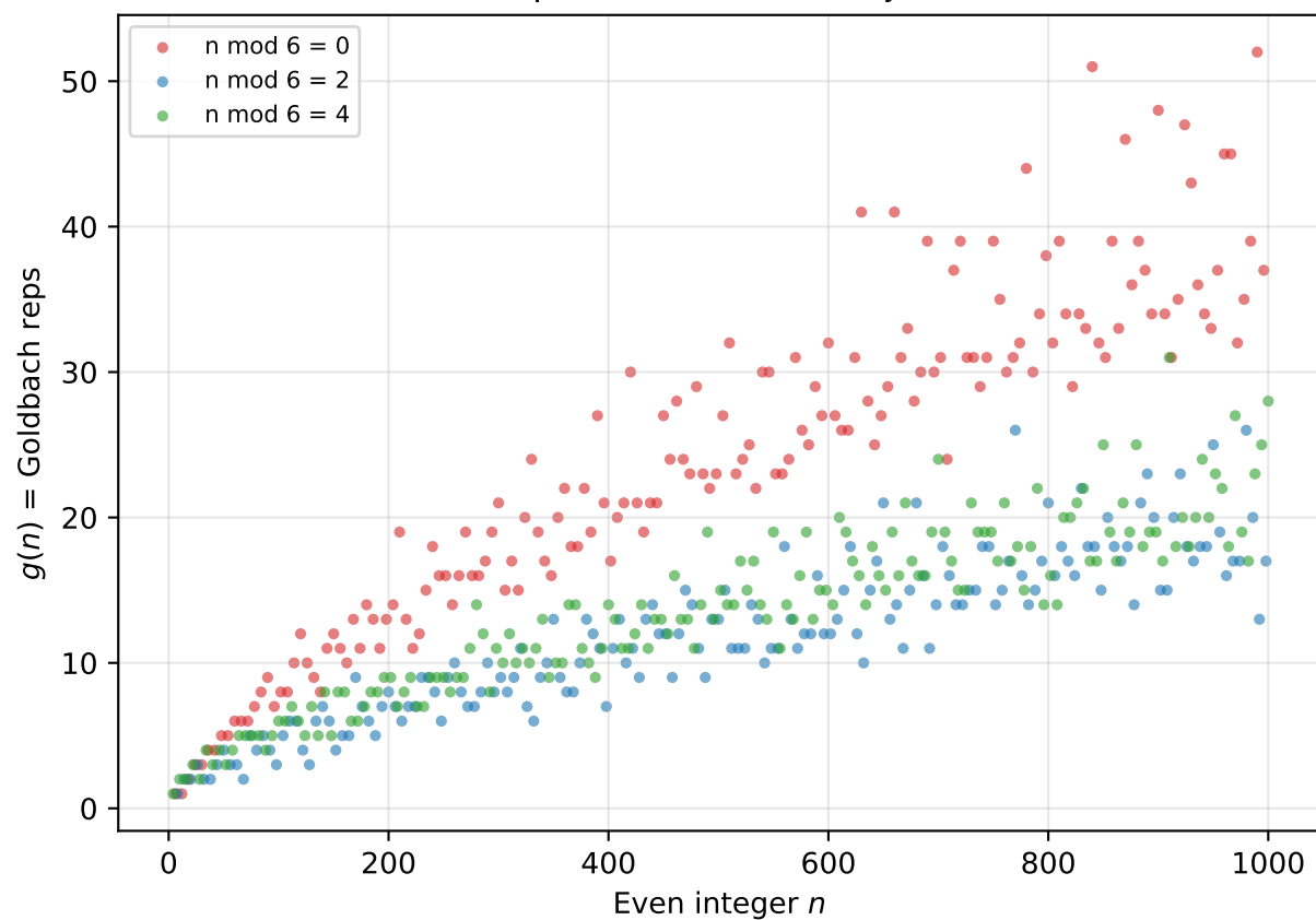
C: Goldbach comet up to n = 1000 — conjecture holds, 3 bands
