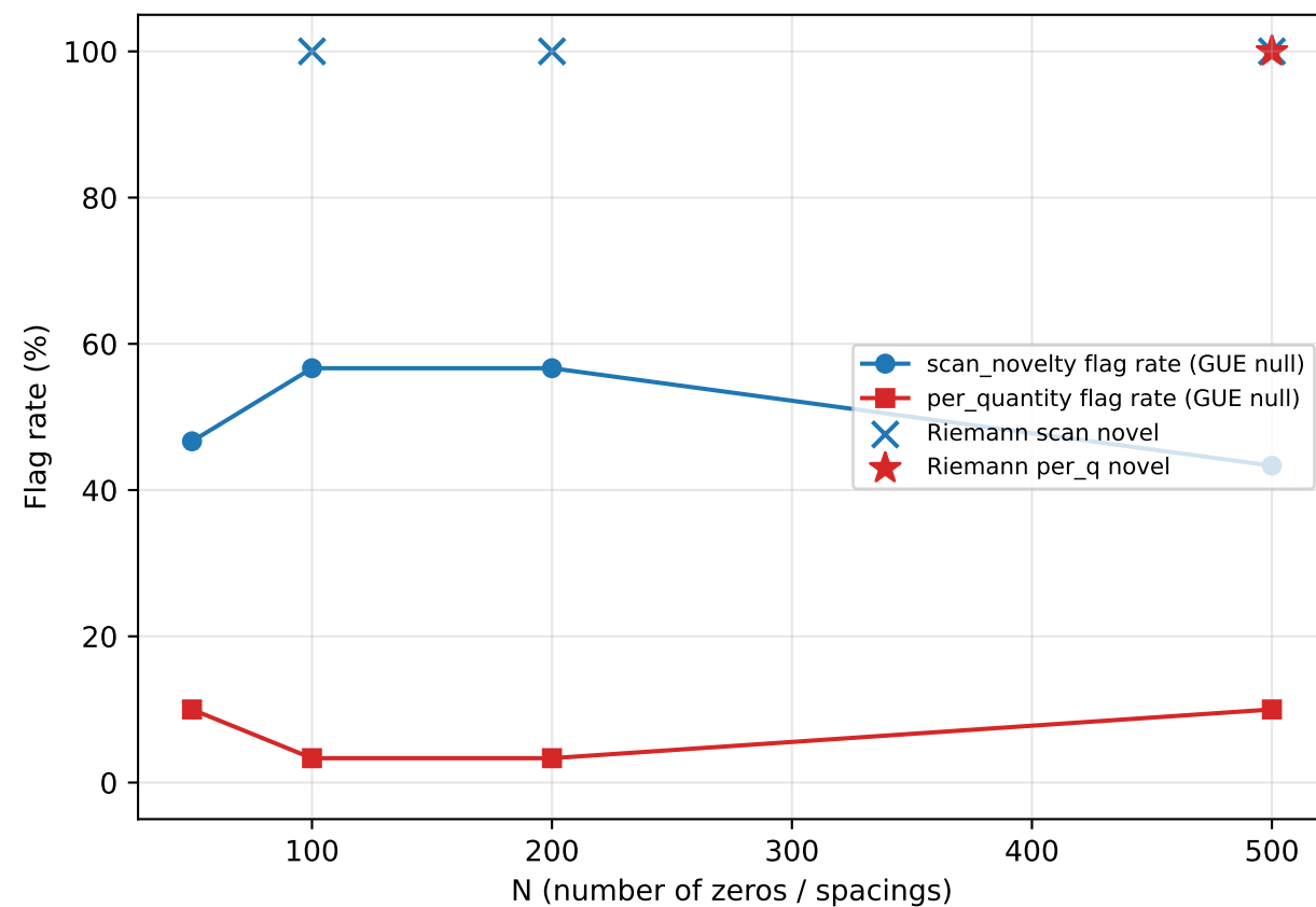
D: GUE null reference — Riemann within finite-N fluctuation
