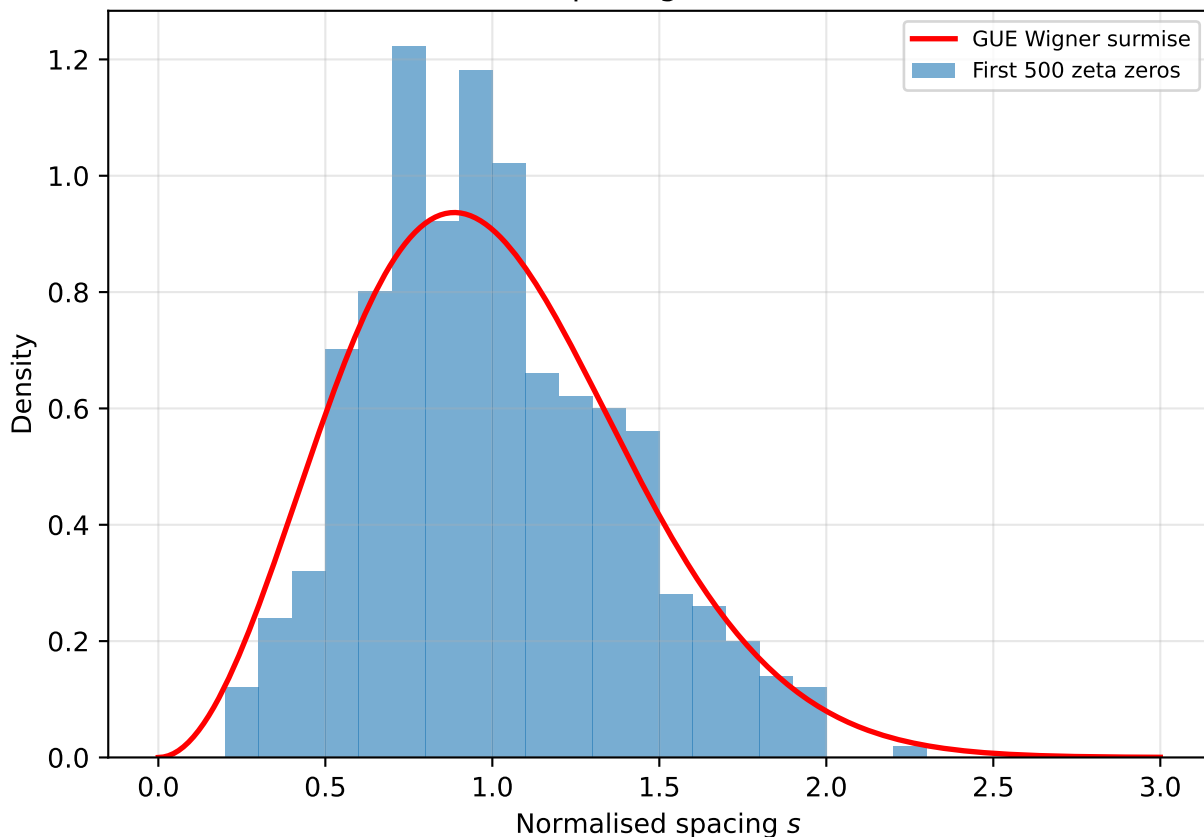
A: Riemann zeta-zero spacings (N=500) — RH-consistent
