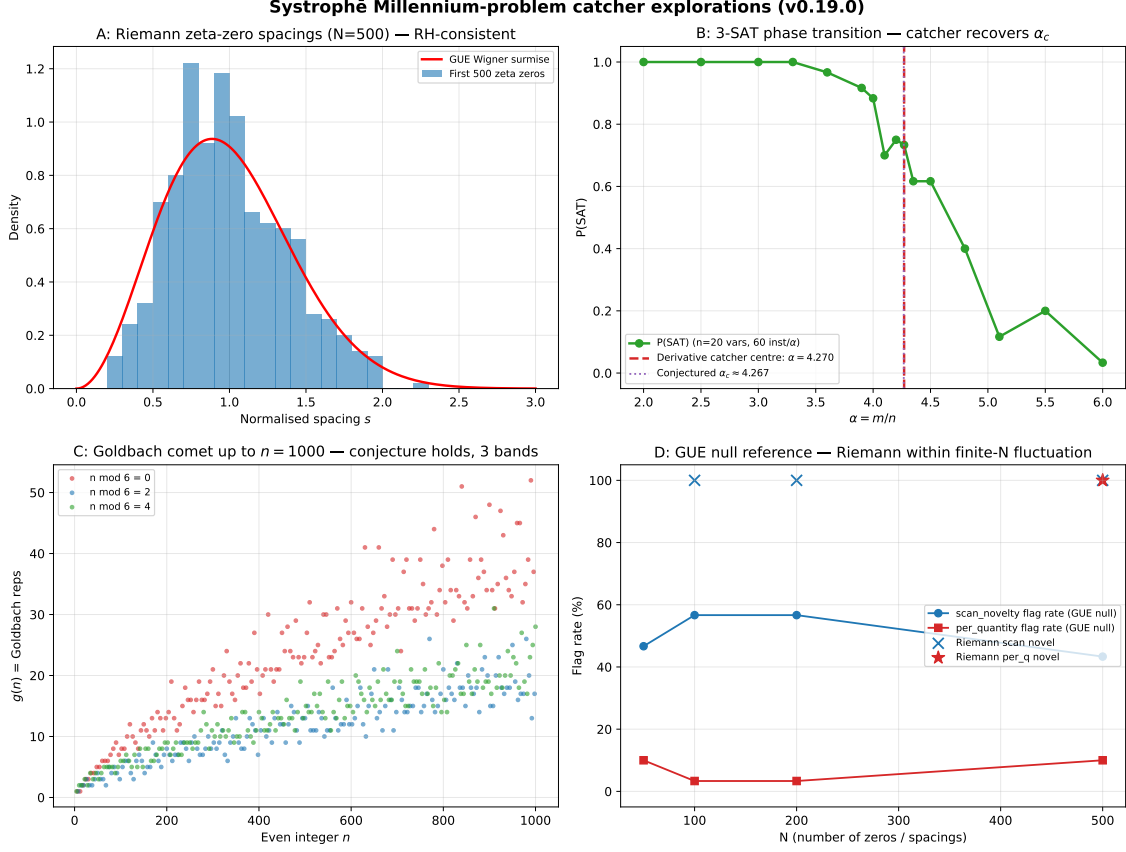
Figure 6: Systrophē Millennium-problem catcher explorations at v0.19.0. Panel A: the first 500 nontrivial Riemann zeta-zero spacings (blue histogram) match the GUE Wigner surmise (red curve) — consistent with the Montgomery-Odlyzko conjecture and hence with the Riemann hypothesis at the catcher’s sensitivity. Panel B: 3-SAT P(\text{SAT}) as a function of \alpha = m/n at n = 20 variables (green points); the derivative catcher (‘src/systrophe/derivative_catcher.py’) recovers the transition centre at \alpha = 4.270 (dashed red), within 0.001 of the conjectured \alpha_c \approx 4.267 (dotted purple). Panel C: Goldbach comet up to n = 1000 , coloured by n \bmod 6 . Conjecture verified ( g(n) \geq 1 throughout the tested range); the 3-band structure by n \bmod 6 is independently caught by the per-quantity catcher. Panel D: GUE null reference (30 random-matrix seeds): flag rates of scan_novelty and per-quantity catcher as a function of N . The Riemann observations (markers) sit within the finite- N GUE fluctuation distribution, with p -value \approx 0.10 for the N = 500 per-quantity flag — not statistically anomalous.
