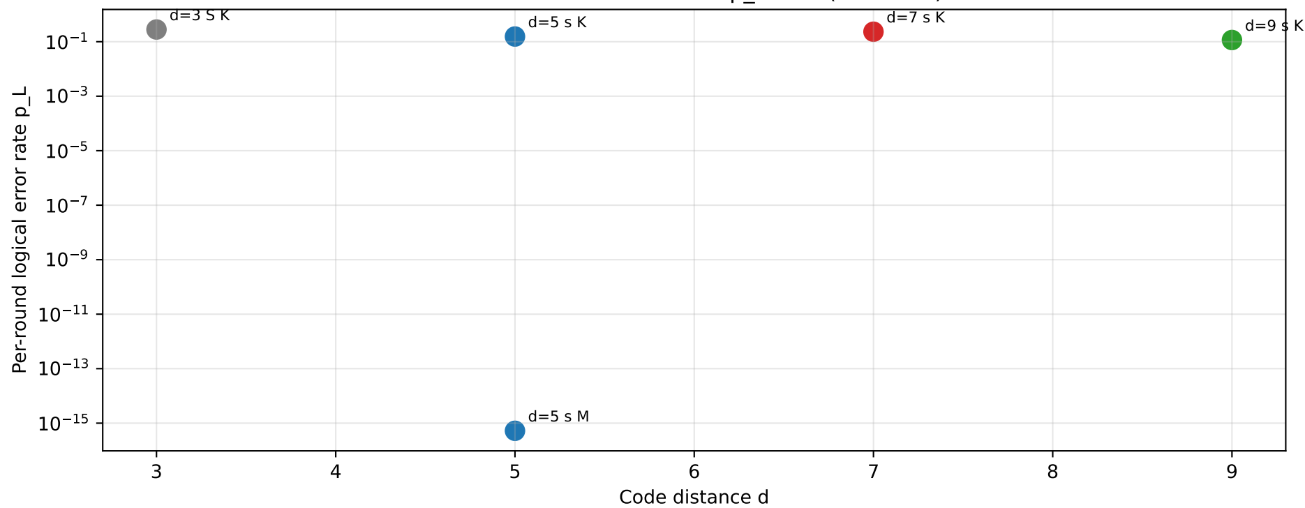
Threshold-theorem view: p_L vs d (Heron-r2)
