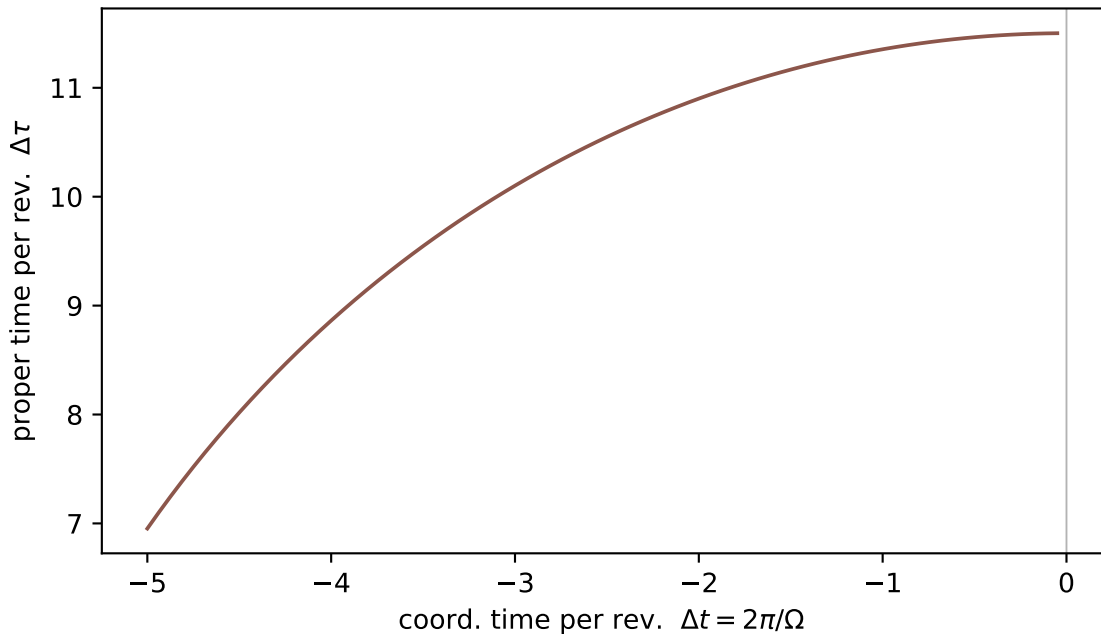
Time-travel orbit (band 1, r \approx 3.35 , a = 1 )
