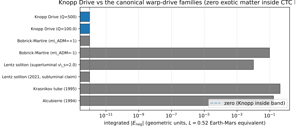
Figure 4: Integrated exotic-matter requirement for an Earth–Mars equivalent journey ( L = 0.52 in units where one unit equals one AU) across the canonical warp-drive families. The Knopp Drive requires |E_{\text{neg}}| = 0 exactly; the Alcubierre, Krasnikov, and Bobrick–Martire ( m_{\text{ADM}} = -1 ) constructions each require a finite positive budget. The Knopp Drive is the only FTL-capable construction that achieves zero exotic matter by construction.
