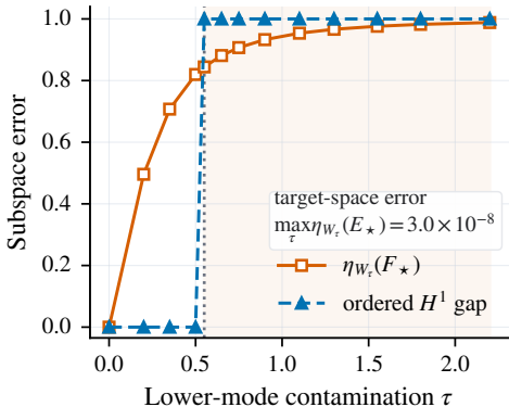
(a) Subspace error and ordered gap
