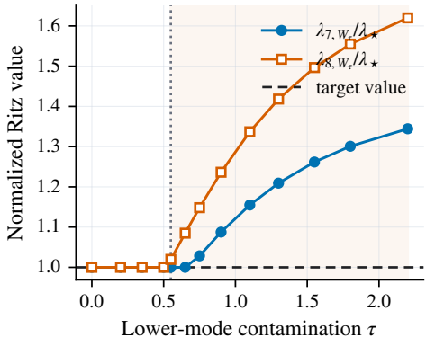
(b) Ordered Ritz values
