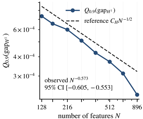
(a) H^1 eigenspace gap
