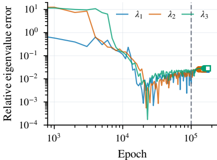
(a) 10D DRM: V(t) = t^2
