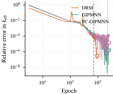
(a) IAEA: k_{\text{eff}}
