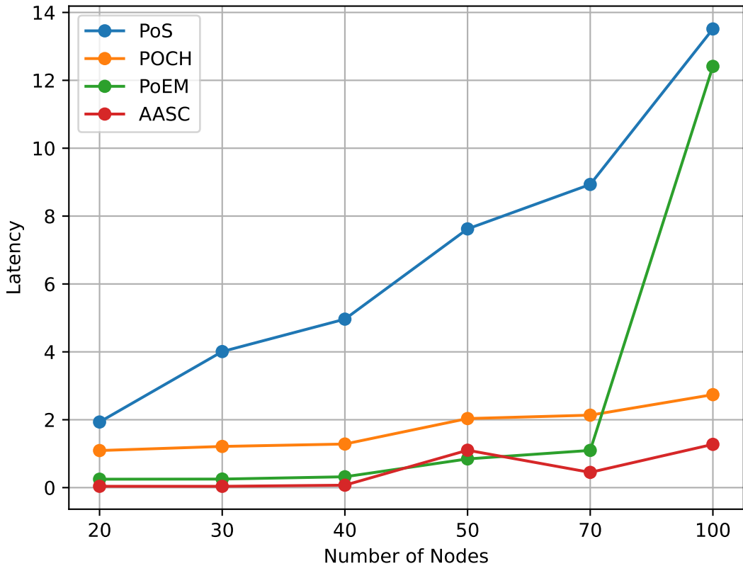
Number of Nodes vs Latency
