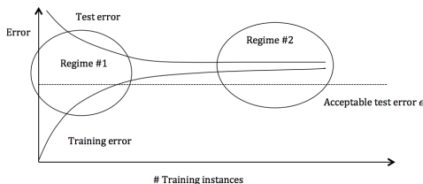
Figure: Given the same model, the changes of training and test error along with the increase of the number of training instances.
