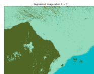
Image segmentation
