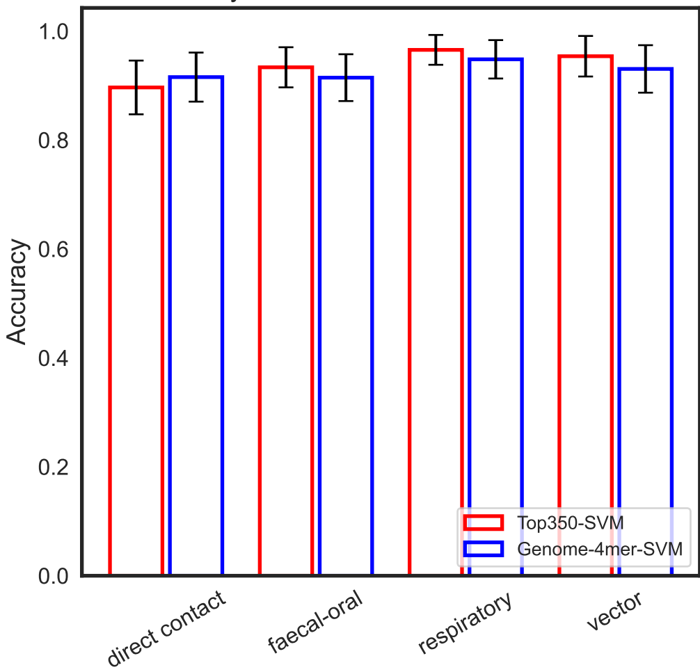
Accuracy Distribution of Transmission Route
