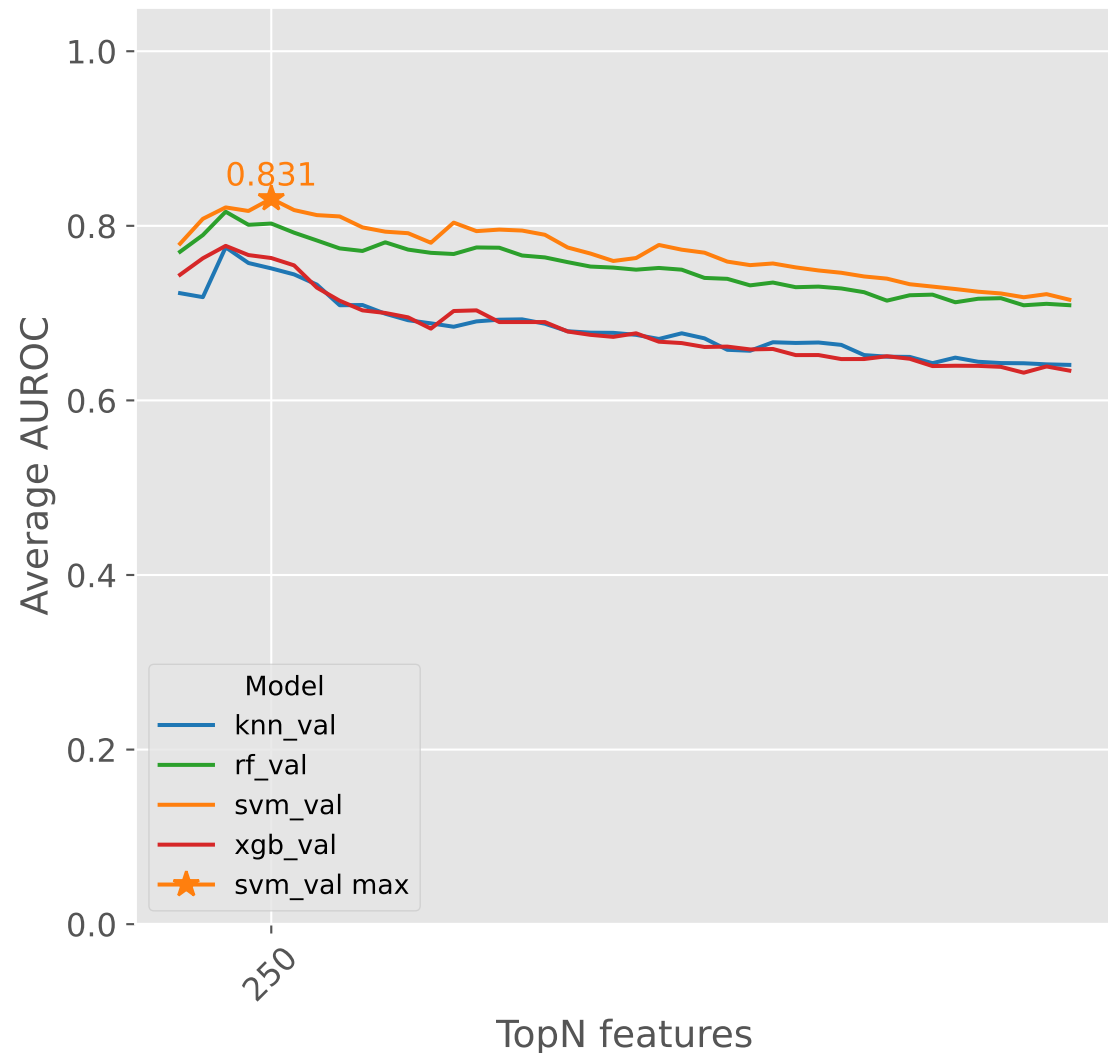
Validation of ML algorithms on Virulence
