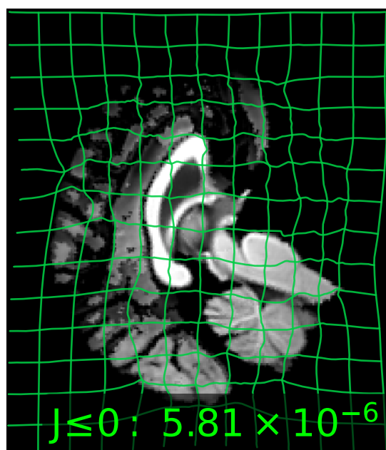
Case B
