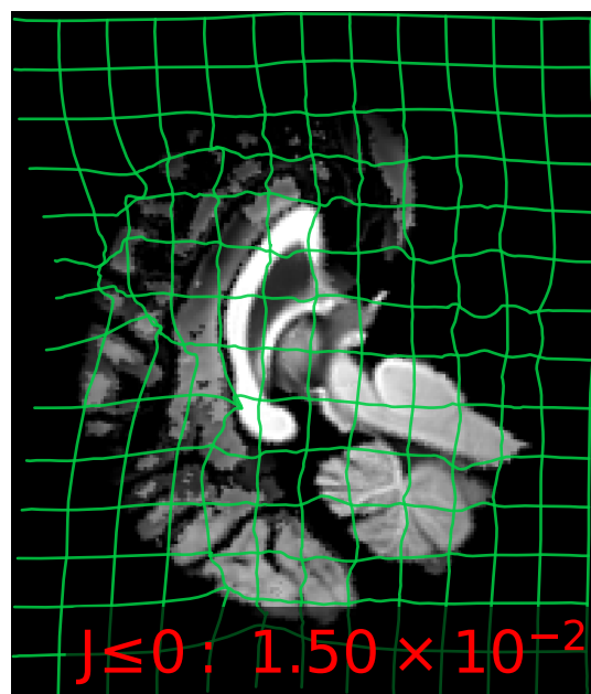
TransMorph
