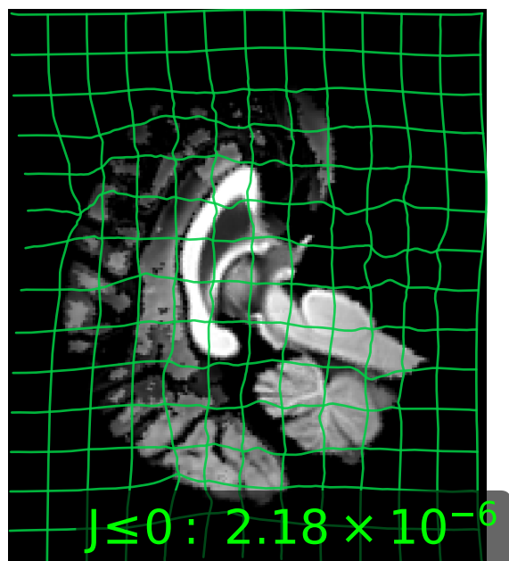
HypEReg-TransMorph
