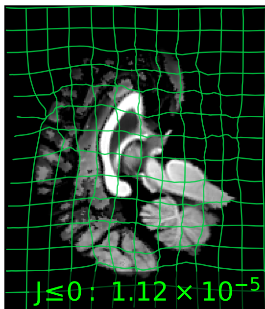
Case C
