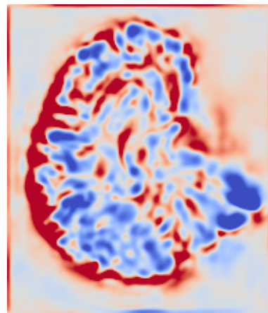
MIDIR Jacobian
