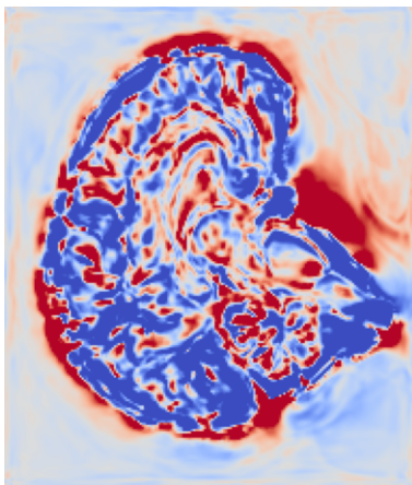
TransMorph Jacobian
