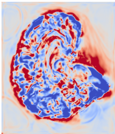
HypEReg-TransMorph Jacobian
