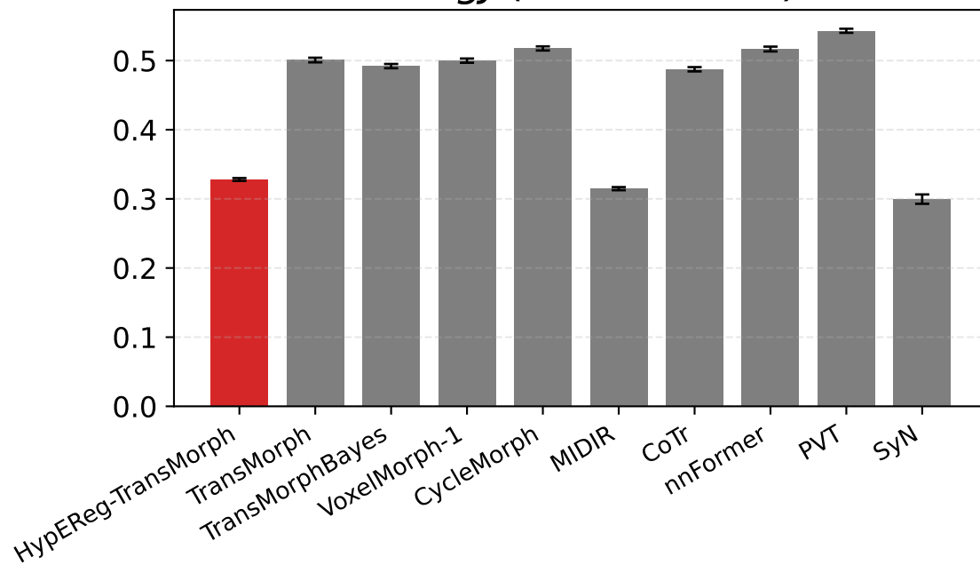
SDlogJ (lower better)
