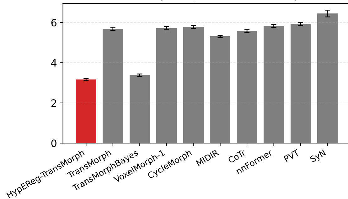
HD95 (mm, lower better)
