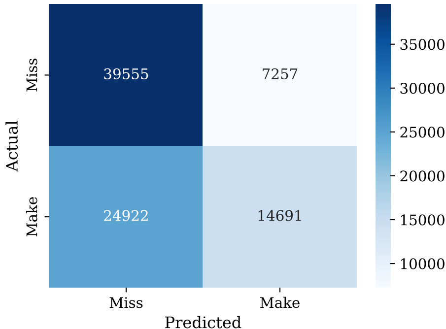
Confusion Matrix — Static-38 + GMM
