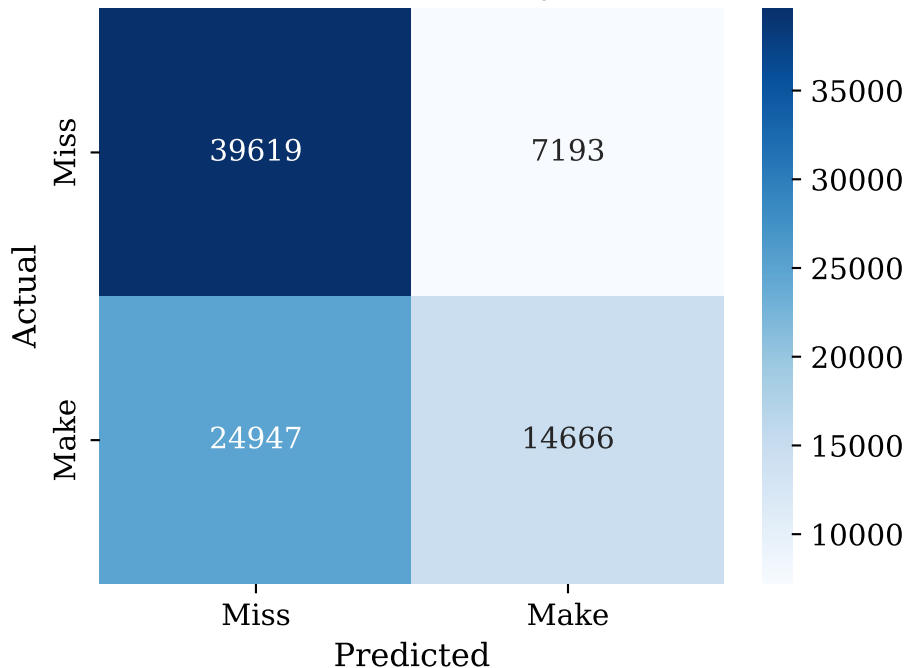
Confusion Matrix — Velocity-65 + GMM
