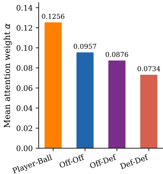
(b) GATv2 Attention
